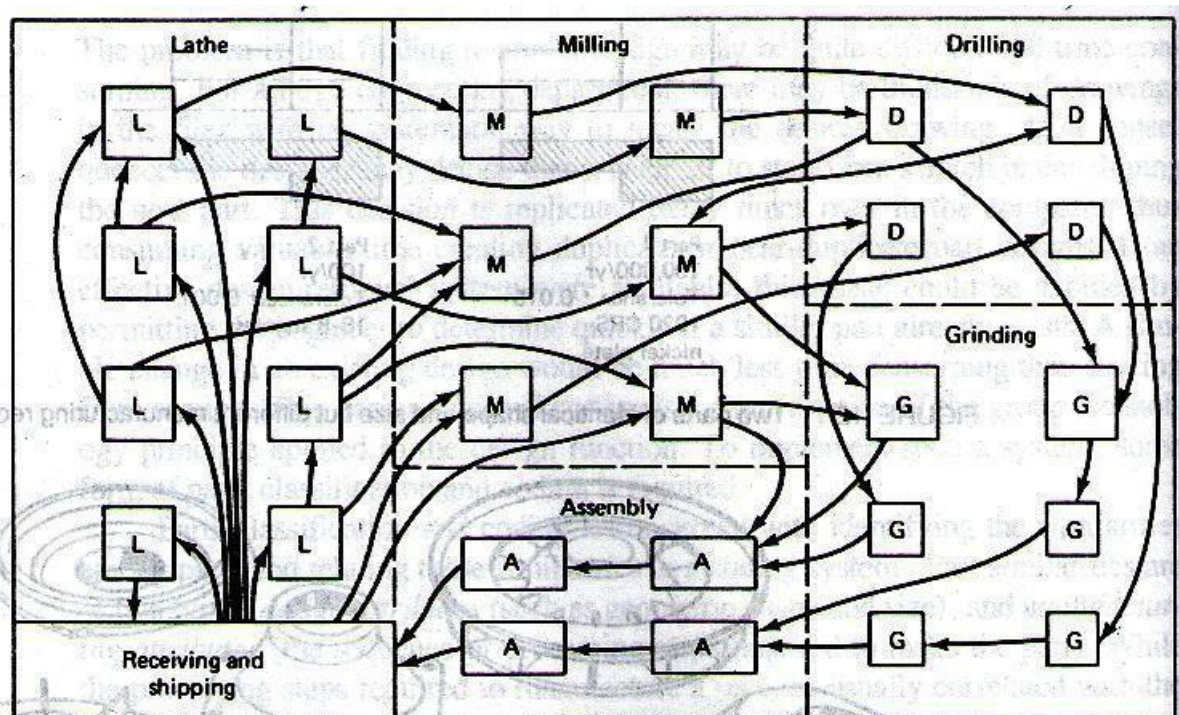
Process-type layout.
