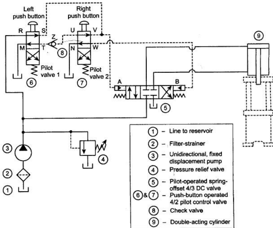
Two Handed Safety Control Circuit
