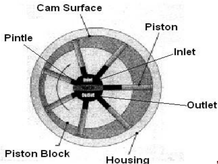
Radial Piston Pump
