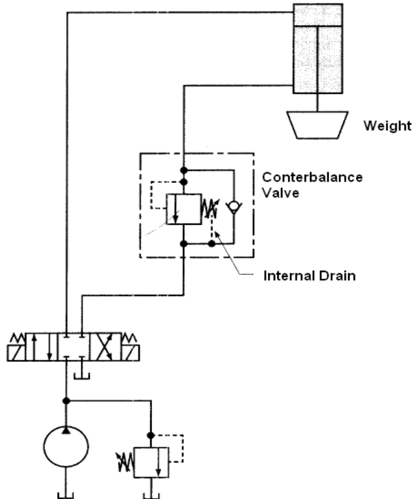
Counterbalance Circuit
