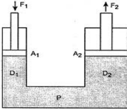
Principle of Bramah's press
