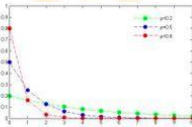
Figure 6A.3: Geometric Distribution
