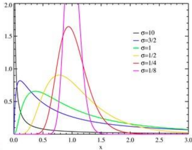
Figure 6A.13: Extreme Value Distributions
