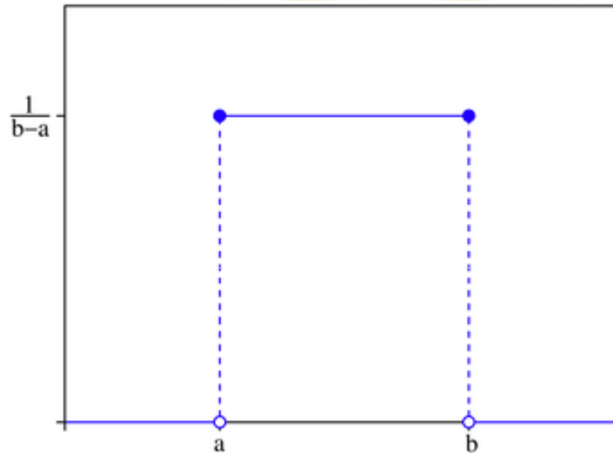
Figure 6A.8: Uniform Distribution
