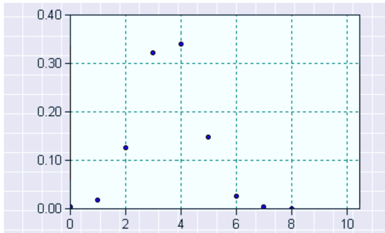
Figure 6A.4: Hypergeometric Distribution
