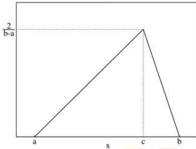
Figure 6A.14: Triangular Distribution
