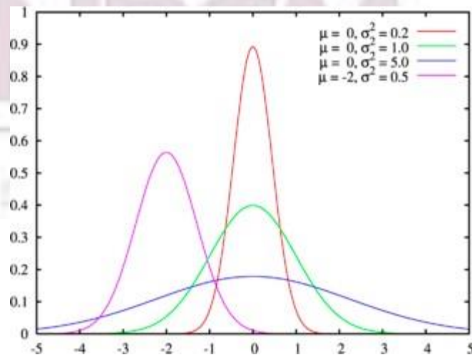
Figure 6A.6: Normal Distribution
