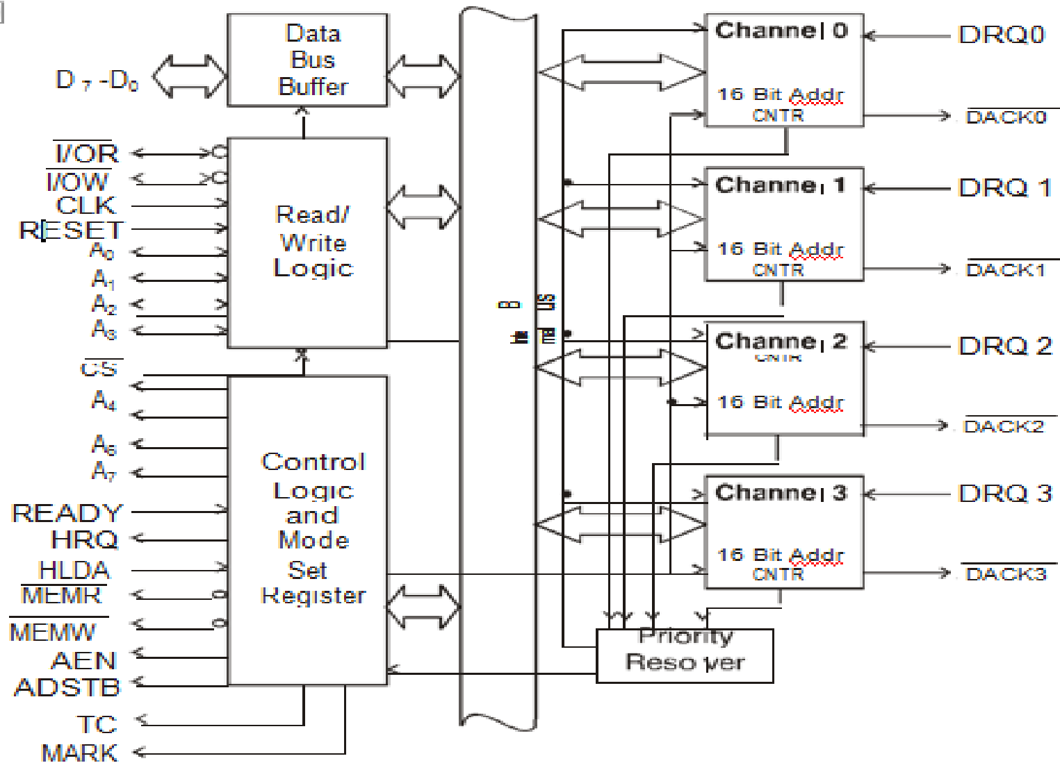
Fig.3.48. Block Diagram
