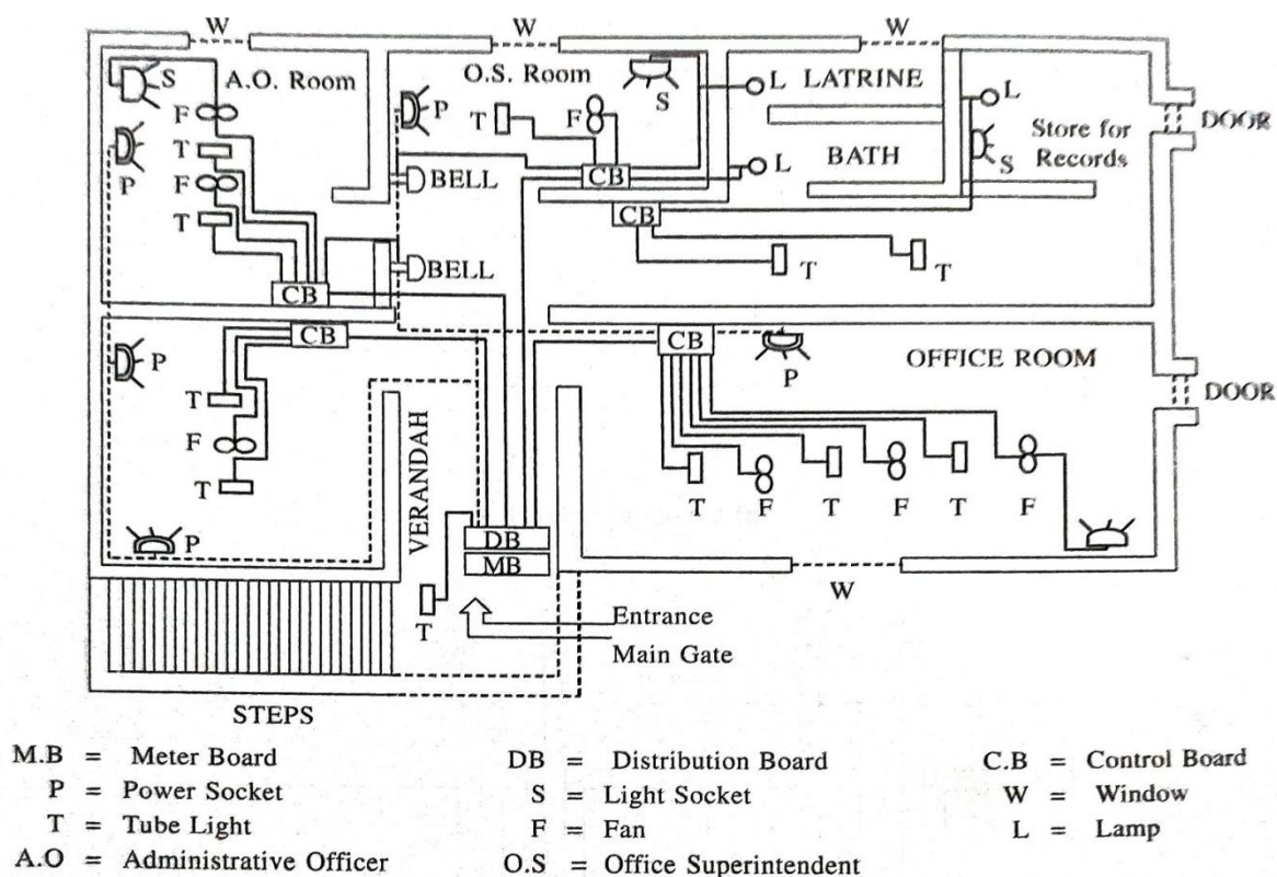
Fig 2.18 : Wiring Layout of a Office
