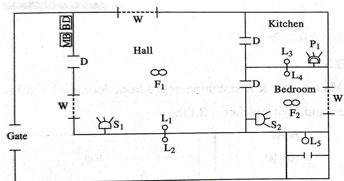
(a) Plan
