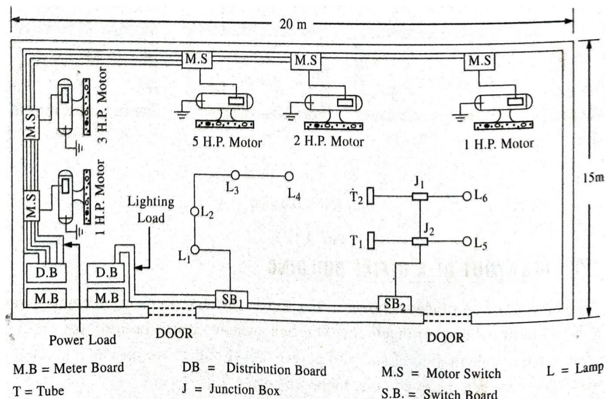
Fig 2.19 : Layout of Work Shop/ Electrical Laboratory
