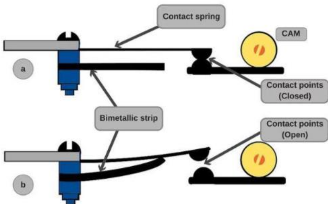
Thermostat
