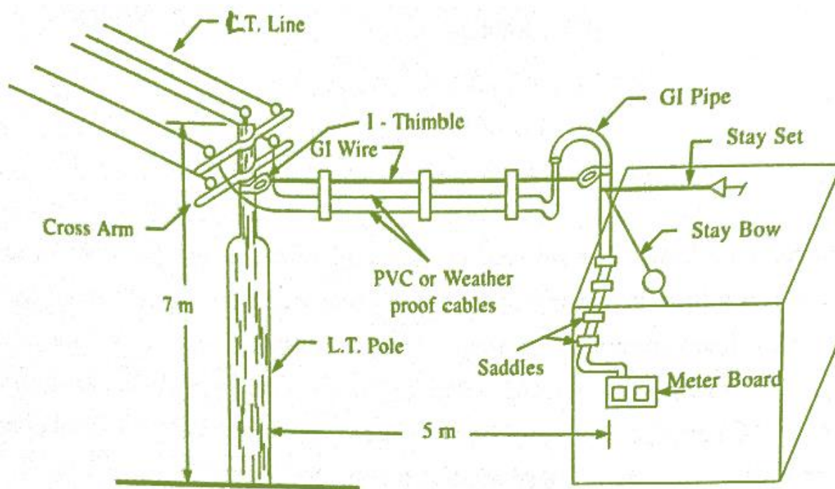
(a) Weather Proof Cable Service Connection
