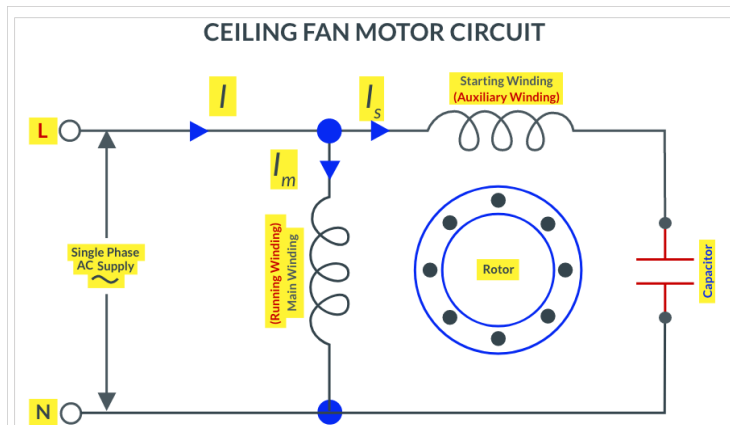
Coil Connection
