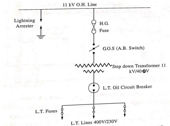
Fig 1 Schematic Diagram of Pole-mounted Sub-station
