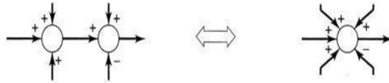
(e) Combining or expanding summations
