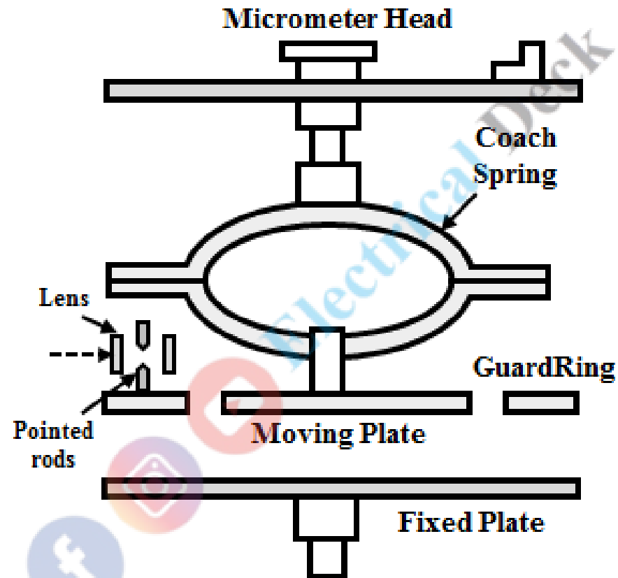
kelvin Absolute Electrometer
