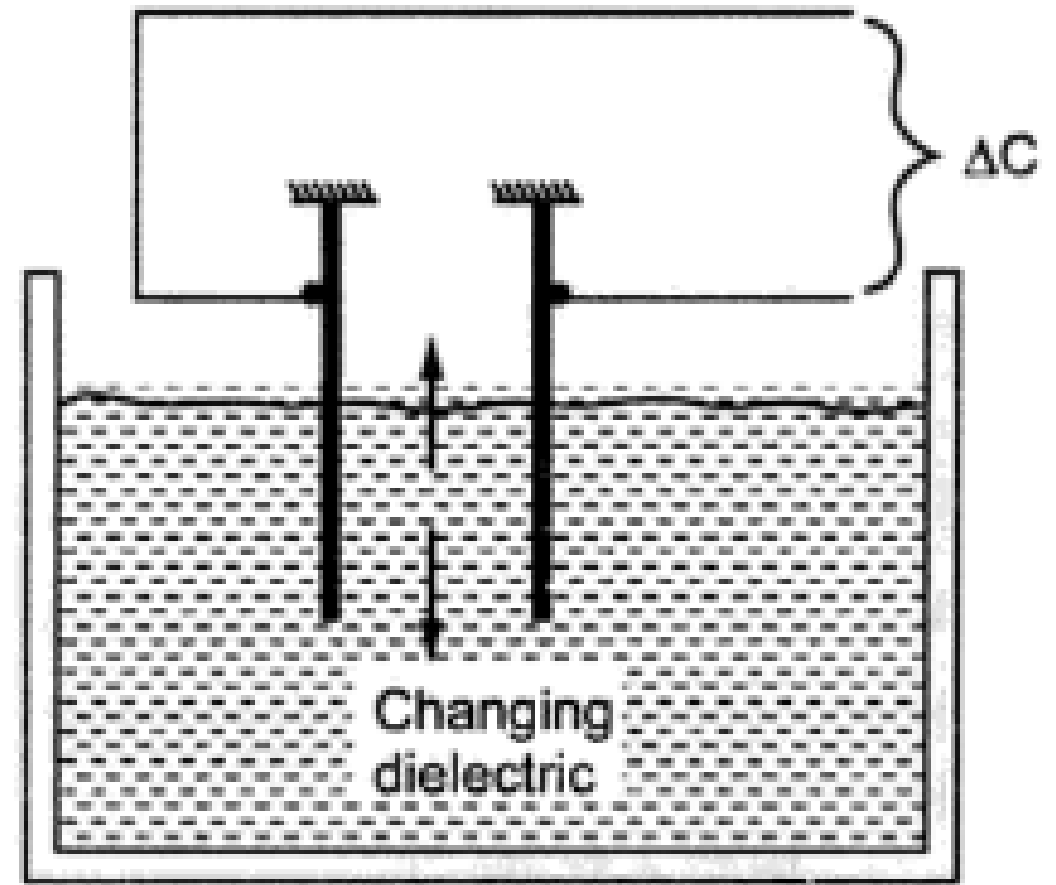
Fig. 9.5 Capacitive transduction
