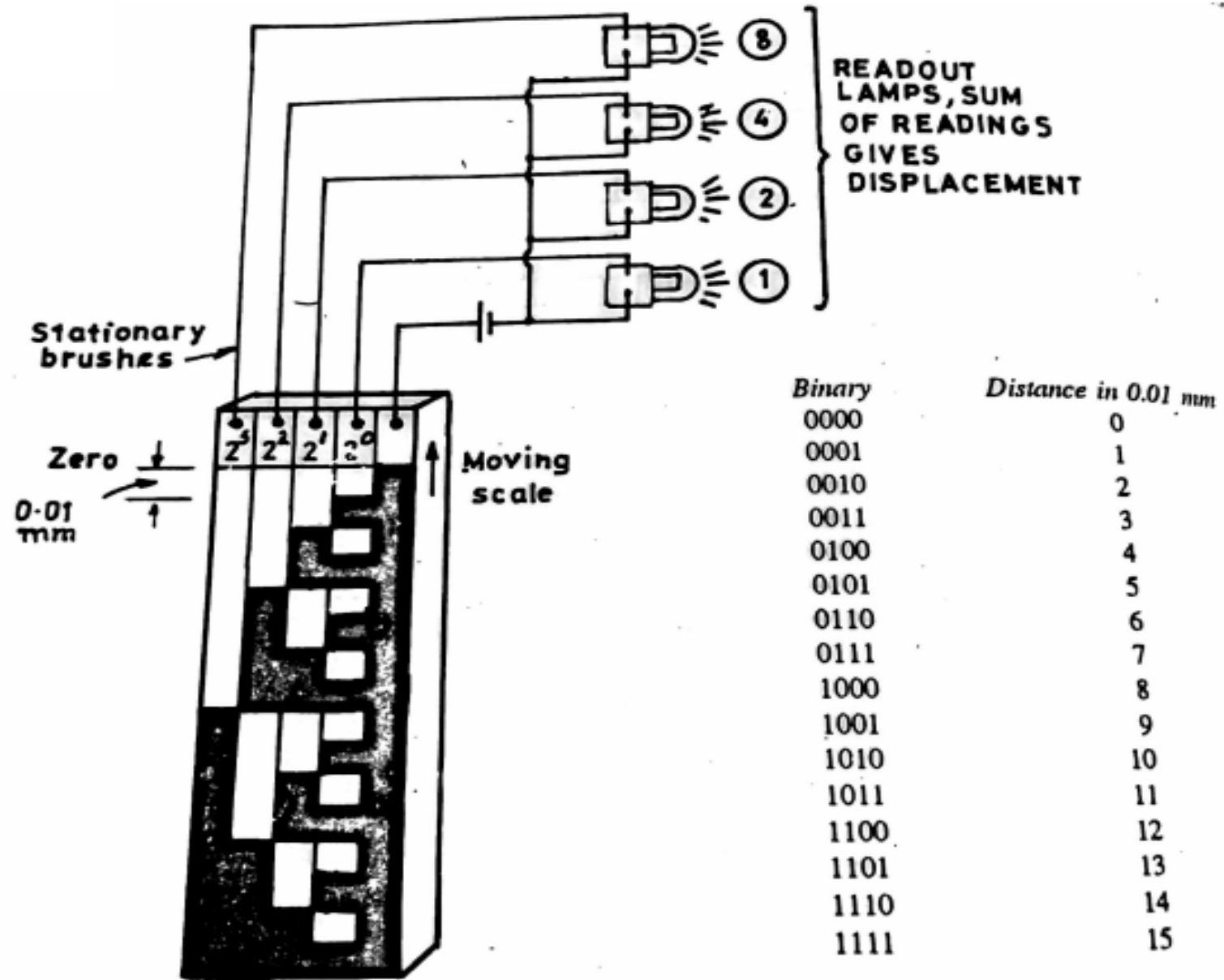
Fig: Translational encoder
