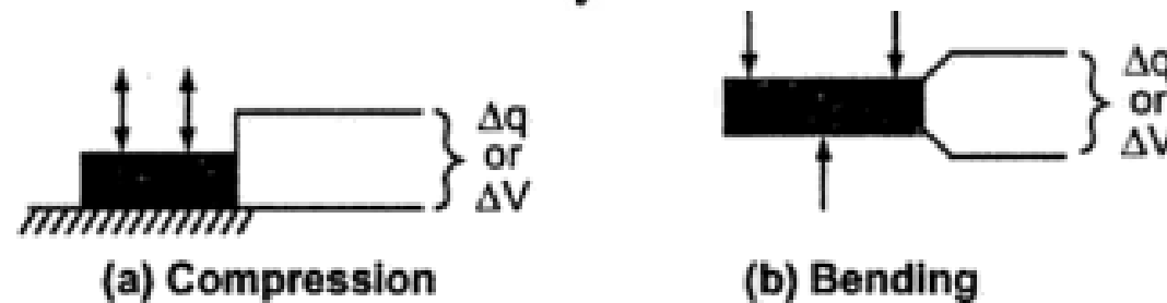
Fig. 9.8 Piezoelectric transduction
