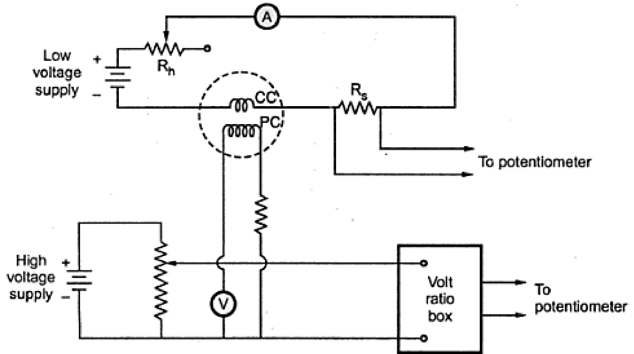
Calibration of wattmeter
