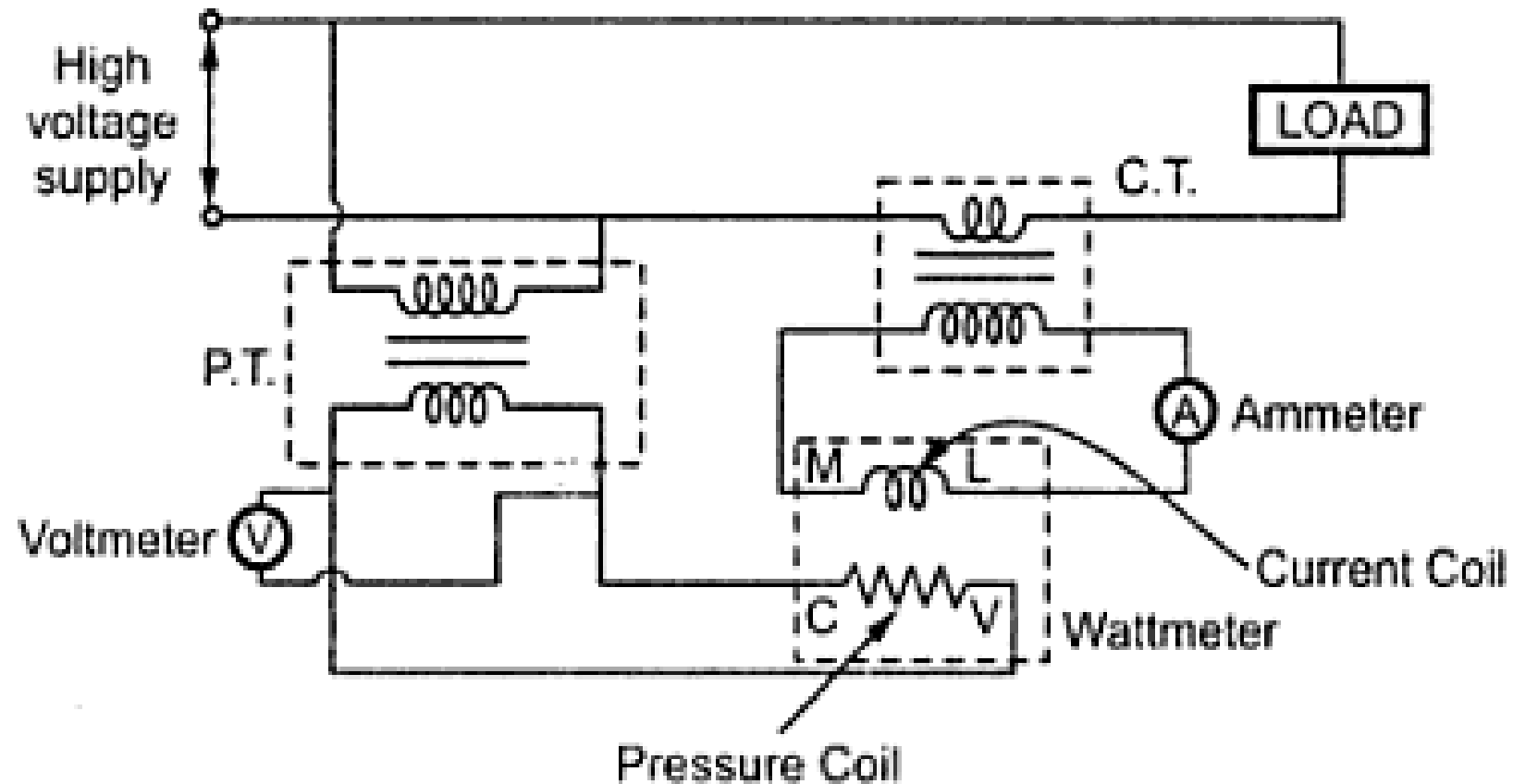
Power measurement using C.T. and P.T.
