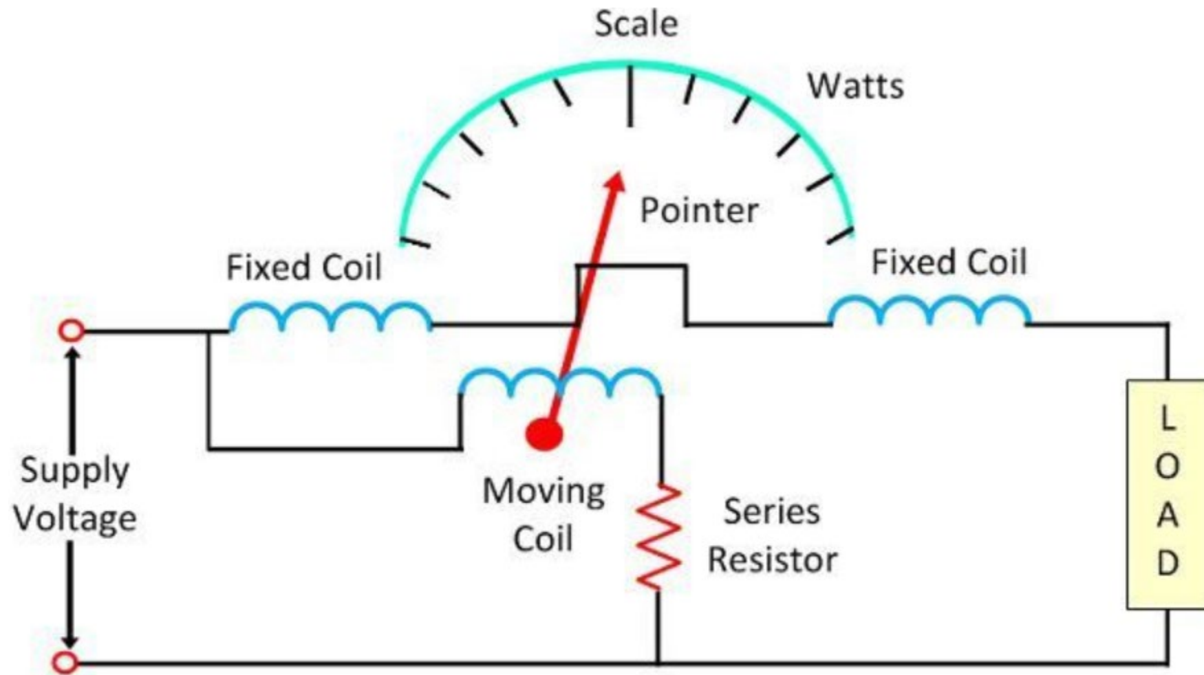
Electrodynamometer Wattmeter
