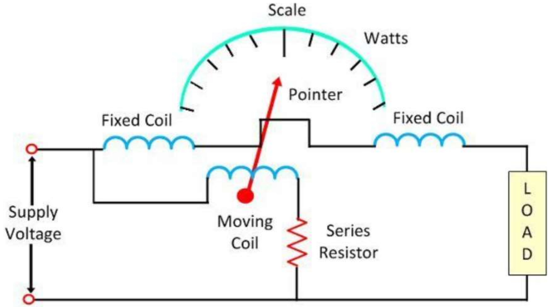
Electrodynamometer Wattmeter
