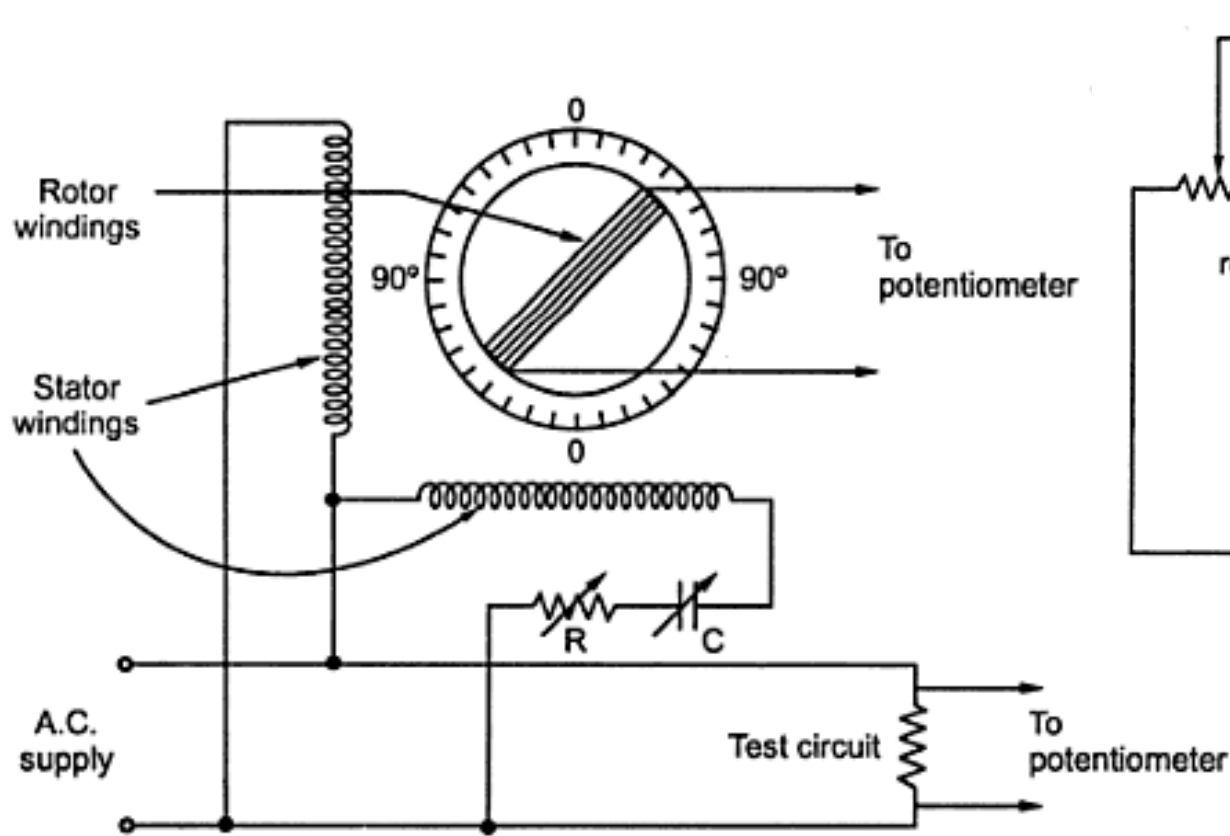
Drysdale phase shifter connection diagram
