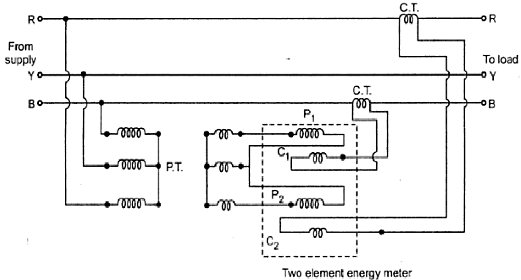
Two element energymeter with C.T. and P.T.
