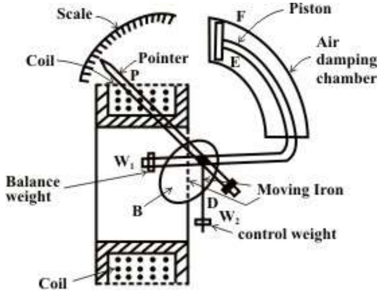
Fig. 42.8: Attraction type
