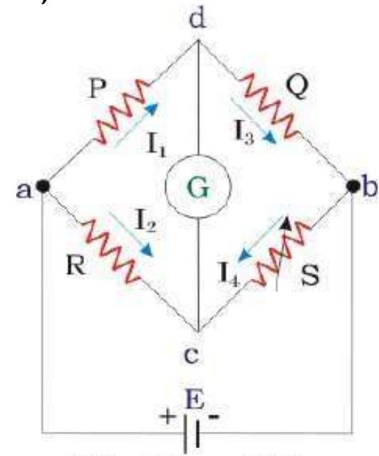
Wheatstone Bridge
