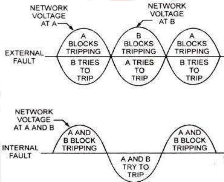
Fig. 5.20. Relations Between Network Output Voltages and Carrier-Current Signals
