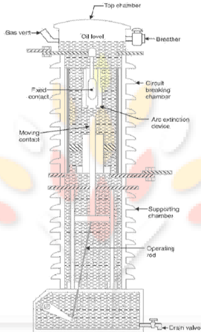
Fig. 19.7 Low-oil Circuit Breaker
