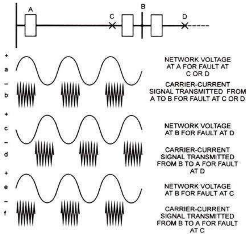
Fig. 5.20. Relations Between Network Output Voltages and Carrier-Current Signals
