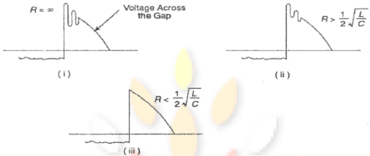
FIGURE 9.9 Transient oscillations for different values of R
