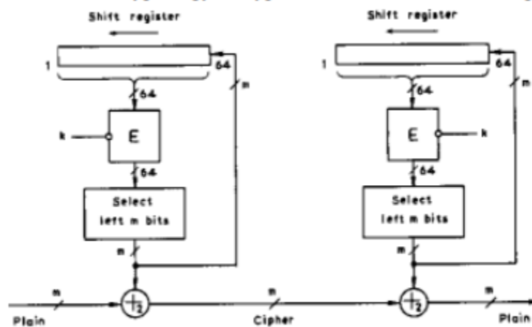
Fig. 4.12 m-bit output feedback
