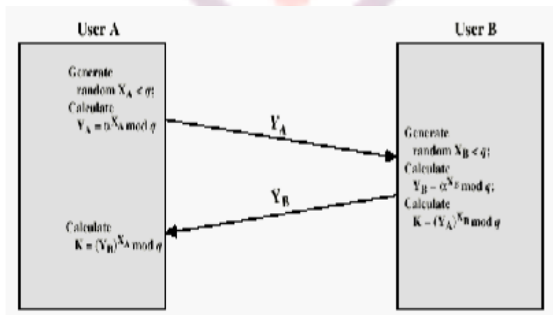
Fig: Diffie-Hellman Key exchange
