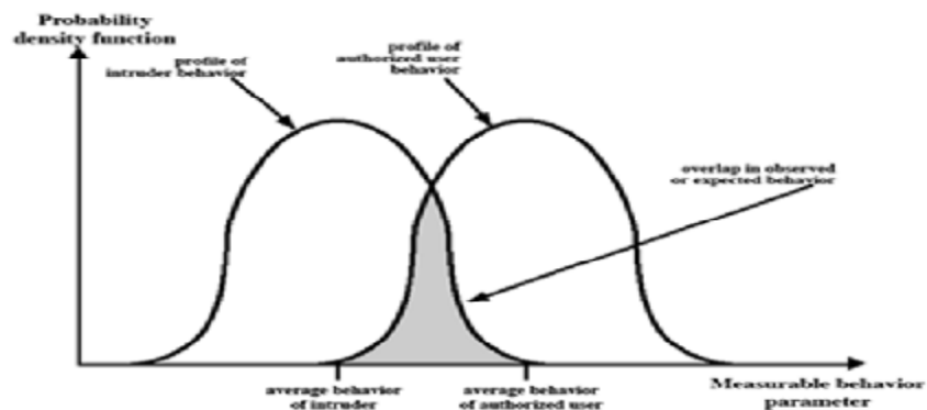
Figure 18.1 Profiles of Behavior of Intruders and Authorized Users
