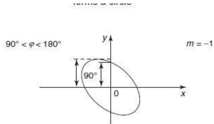
Figure 14-13 Lissajous figure when 90 < \varphi < 180
