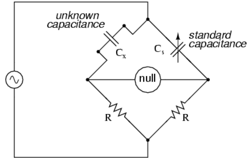
capacitance
