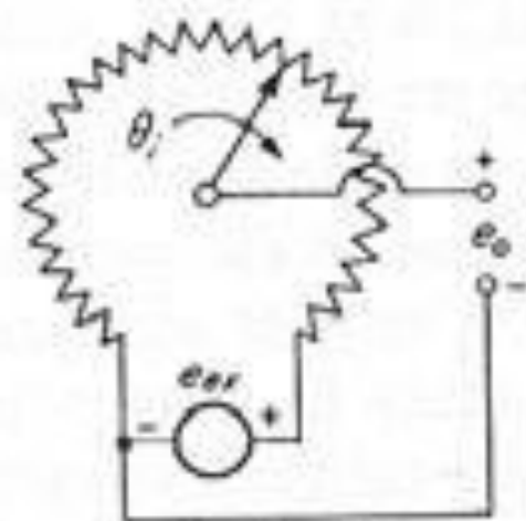
Single-turn
