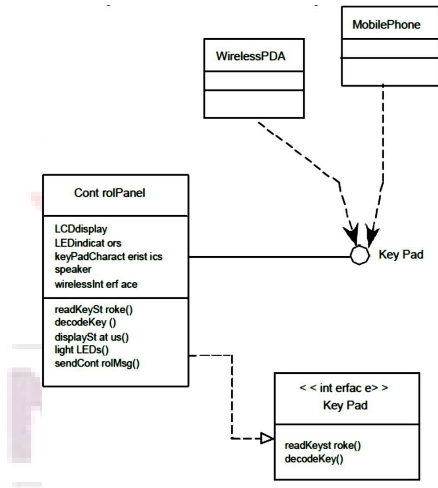
Figure 9.6 UML interface representation for Control Panel
