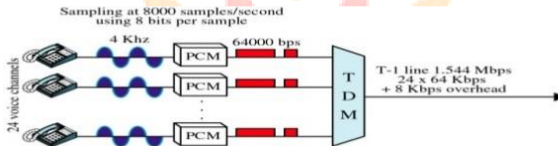
Fig 1: T1 digital system
