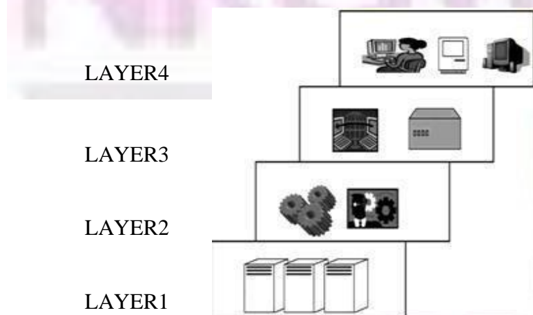
FIGURE 3.2 Cloud Layers.
