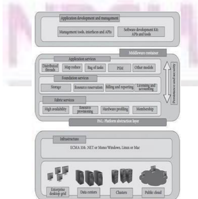
FIGURE 5.5 Overview of the Aneka platform
