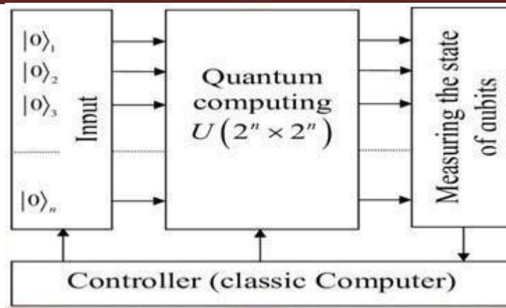
Fig9 Quantum Computing
