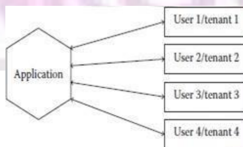
FIGURE3. Multitenancy.
