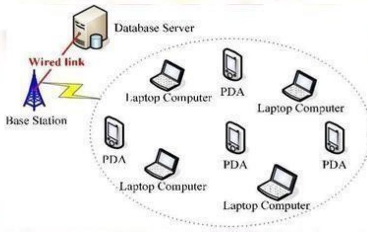
Fig8MobileComputing
