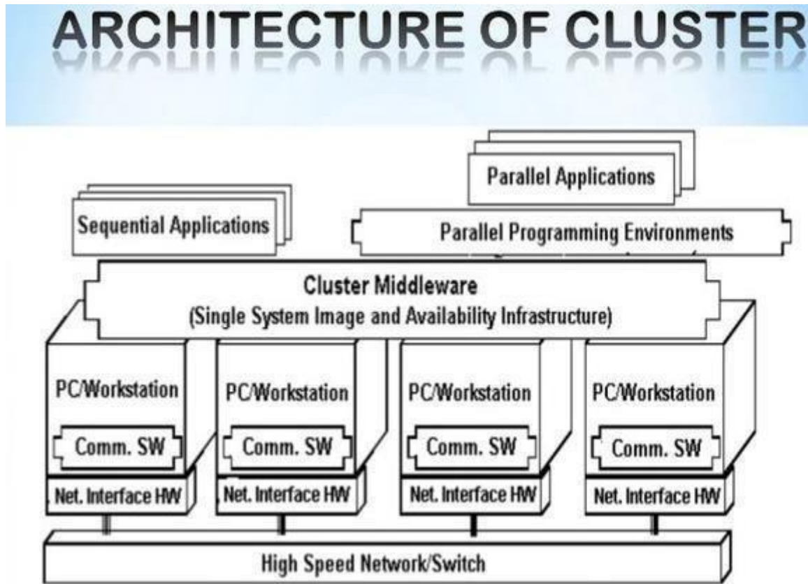
Fig4Cluster Computing
