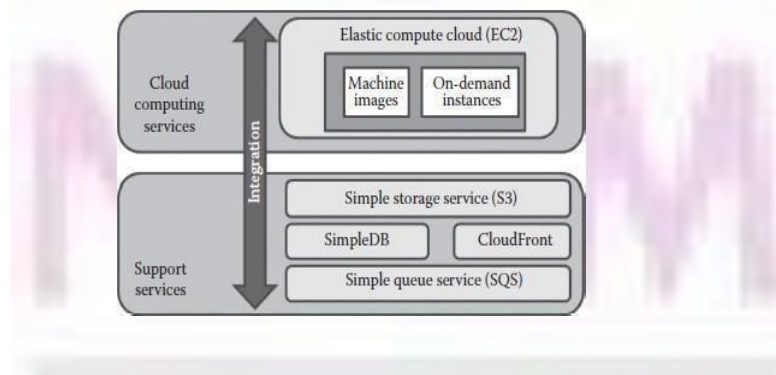
FIG5.3-AWS
