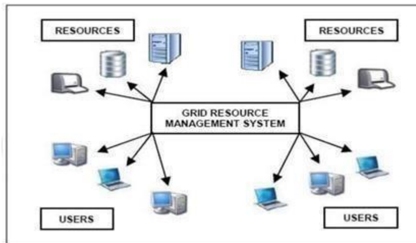
Fig5 Grid Computing
