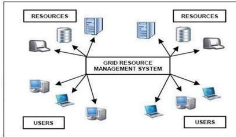
Fig5 Grid Computing
