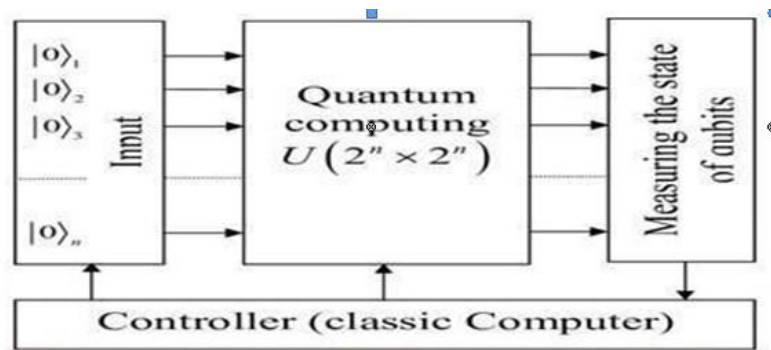
Fig9 Quantum Computing
