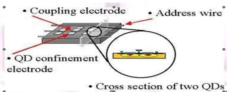
Fig10 Optical Computing
