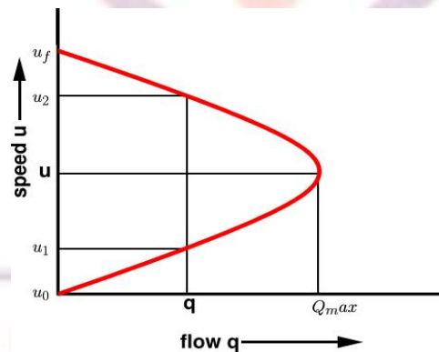
Fig.15 Speed-flow diagram
