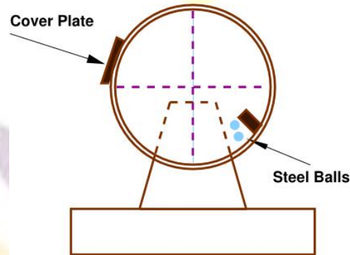
Fig.26 Los Angeles abrasion test setup
