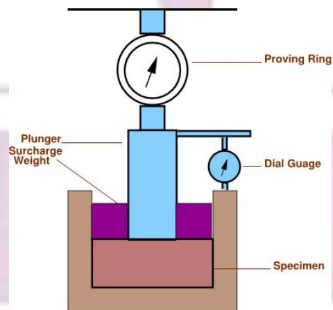
Fig 23 CBR Test
