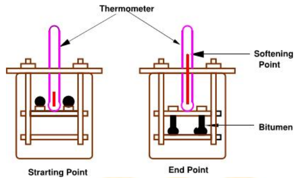
Fig. 32 Softening Point Test Setup
