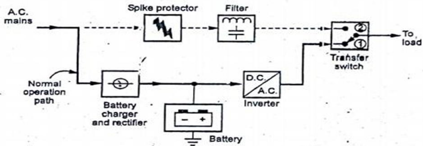
Online UPS
