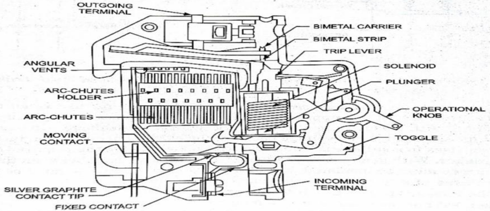
Miniature Circuit Breaker
