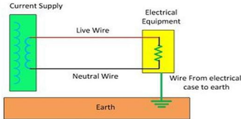
Earthing
