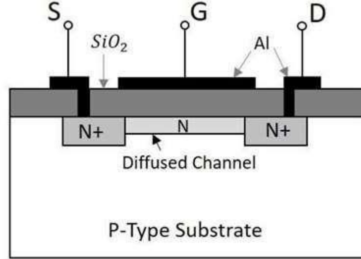
Structure of N-channel MOSFET
