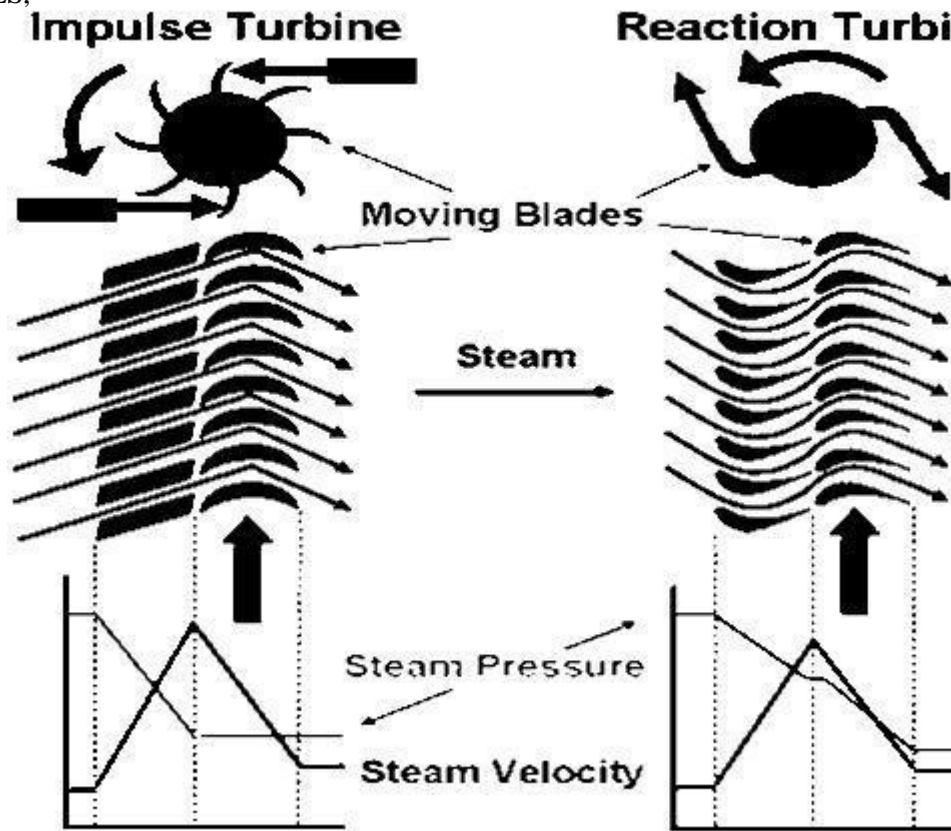
impulse turbine and reaction turbine pressure and velocity diagram
