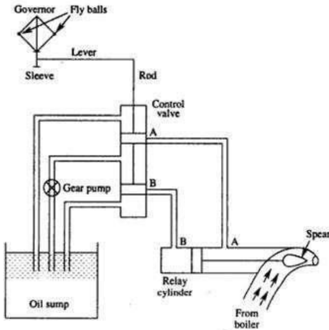
Fig 3.14 Throttle Governing
