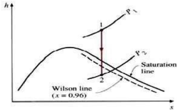
The h - s diagram for the isentropic expansion of steam in a nozzle.
