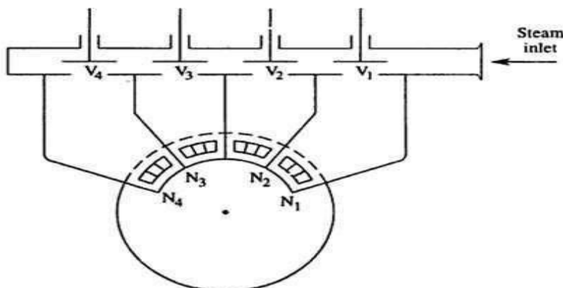
Fig 3.15 Nozzle Governing
