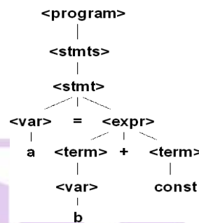
Figure 2.1 Parse Tree
