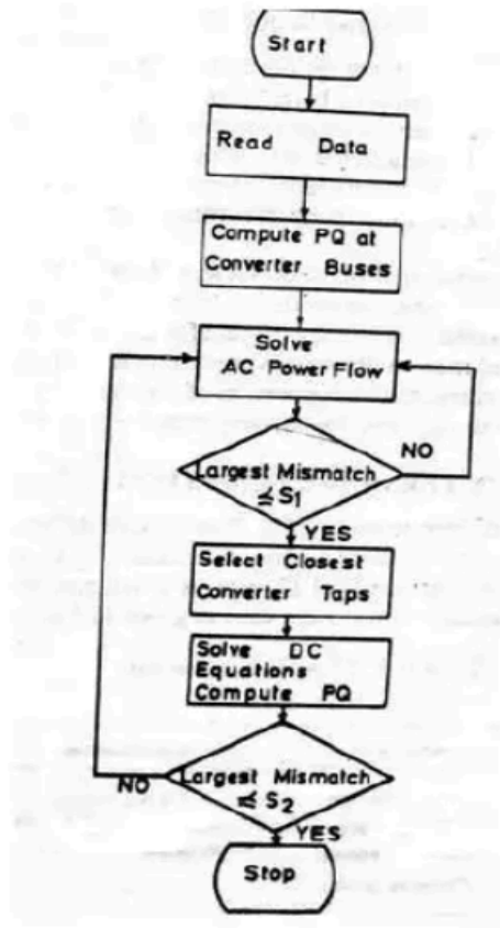
Flow chart of AC/DC Load Flow
