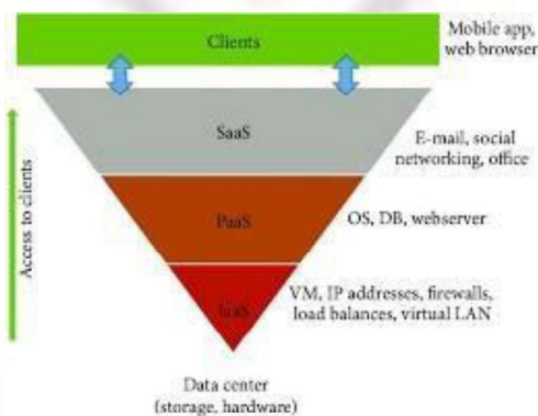
FIGURE 2.3 SPI—service offering model of the cloud.
