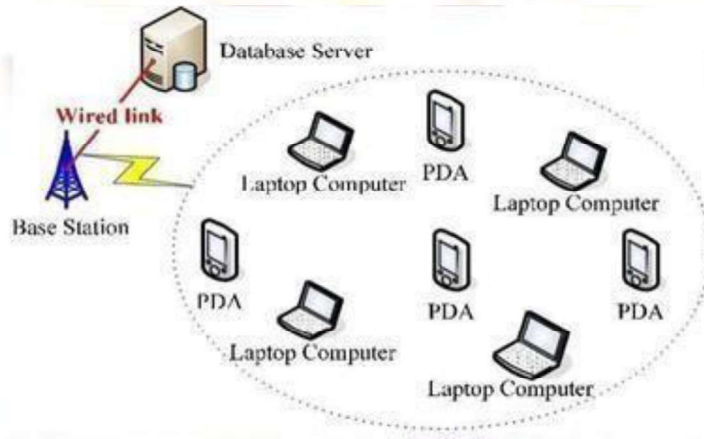
Fig 8 Mobile Computing
