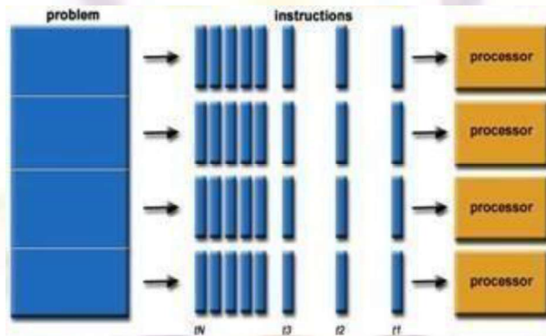
Fig 2 Parallel Computing
