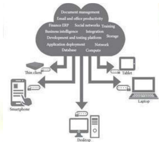
FIGURE 2.1 Cloud computing
