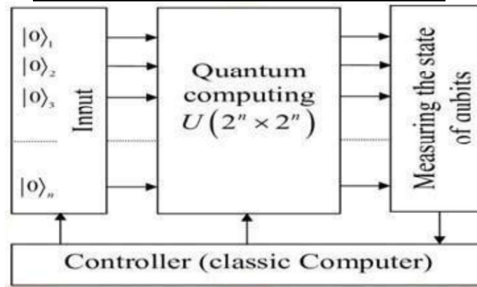
Fig 9 Quantum Computing
