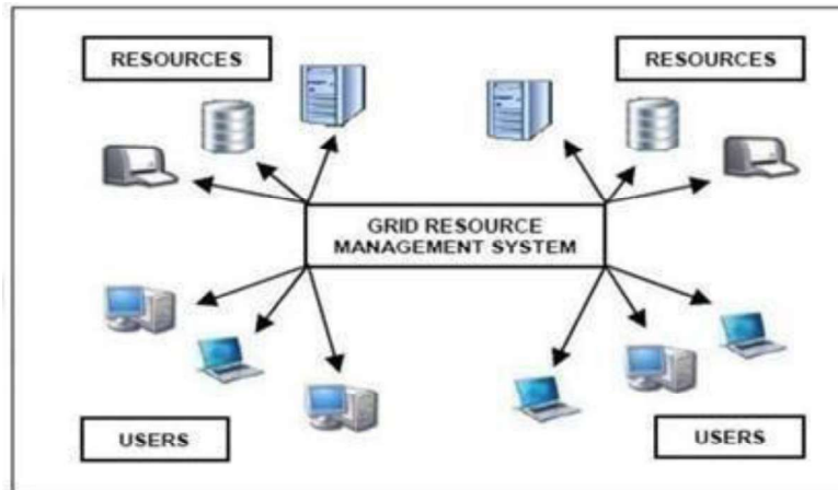
Fig 5 Grid Computing
