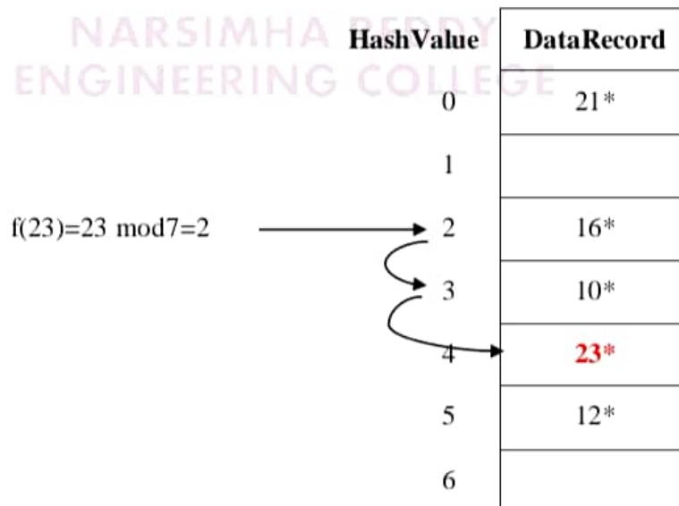
Figure5.2: Linear Probing
