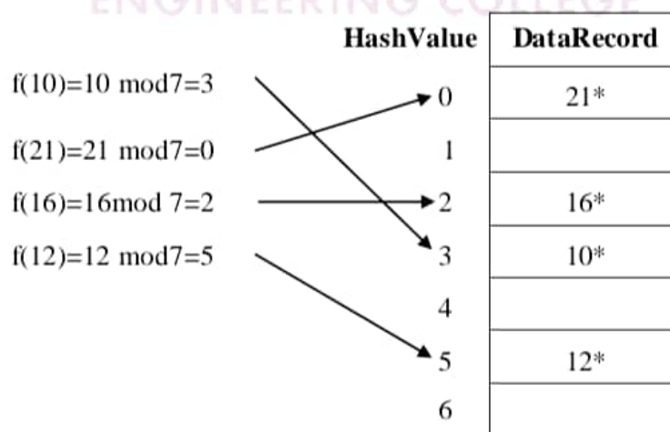
Figure 5.1: Static hashing
