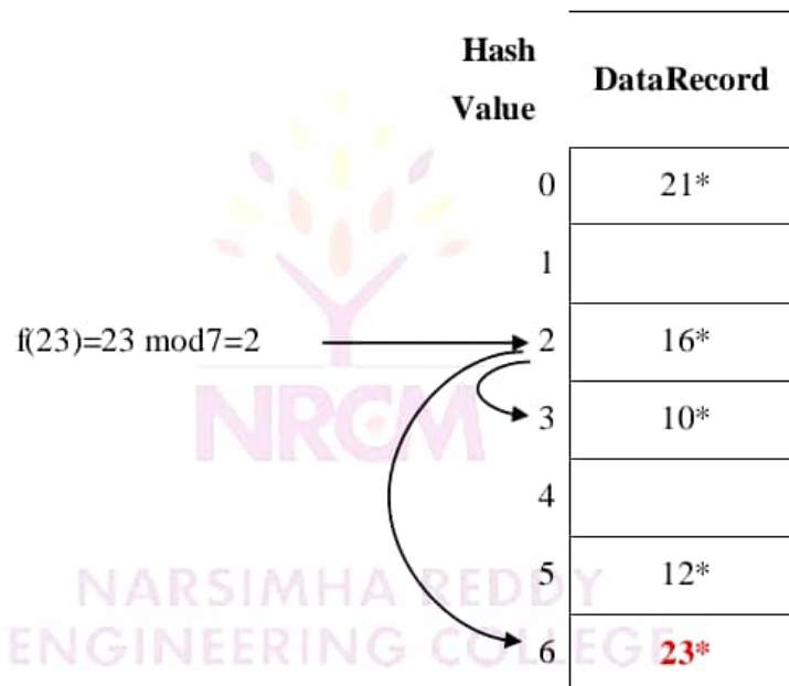
Figure 5.3: Quadratic Probing
