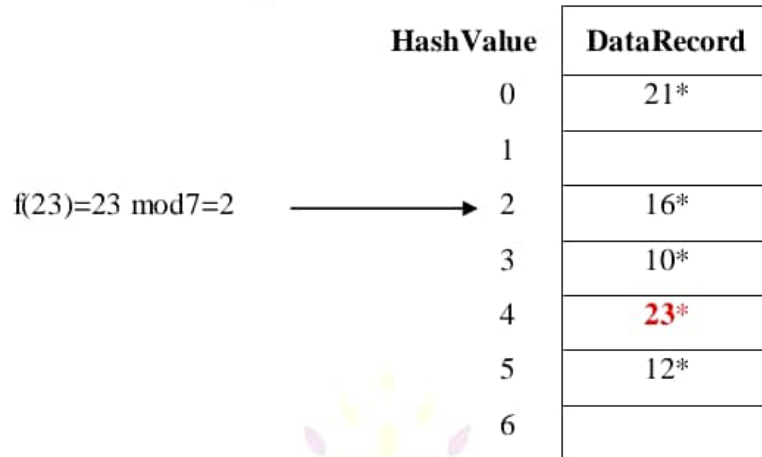
Figure 5.4: Double Probing
