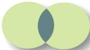
INNER JOIN
