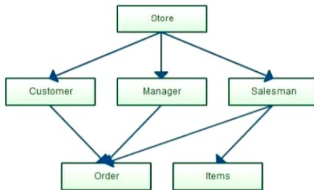
Figure:NetworkModel
