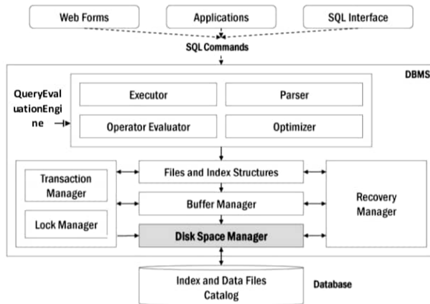
Figure:DBMS Structure
